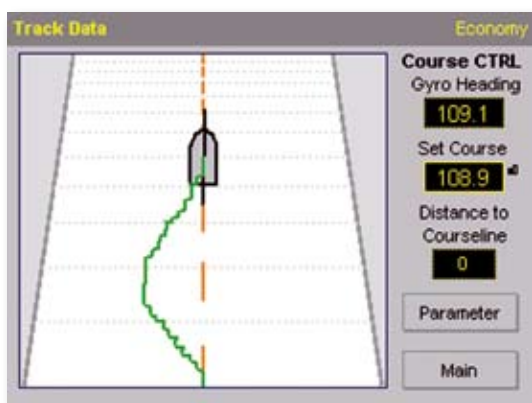
NautoPilot® 5000 illustrates graphically any deviations from the course over ground line
