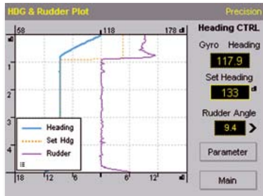
Rudder activity and heading changes are displayed. Autopilot settings can directly be changed
