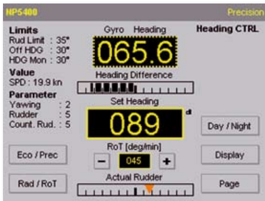
NautoPilot® 5000 main screen with touch operation
